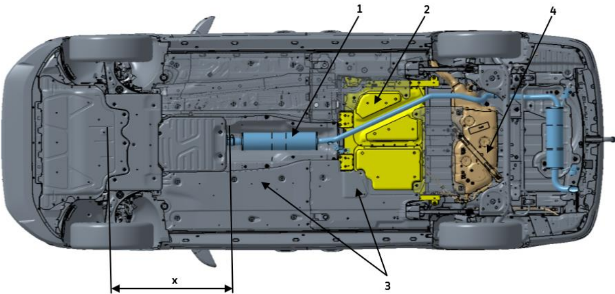
Fig. 2: PHEV exhaust system, long wheelbase (illustration: drive type 4x2, 85KW TSI)
