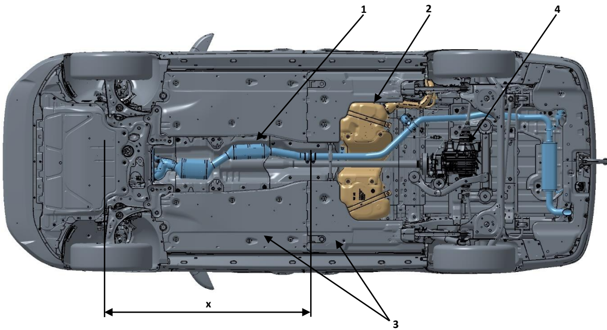
Fig. 2: 4x4 drive exhaust system (all-wheel drive), long wheelbase (illustration: 4x4 drive type, 90KW TDI)
