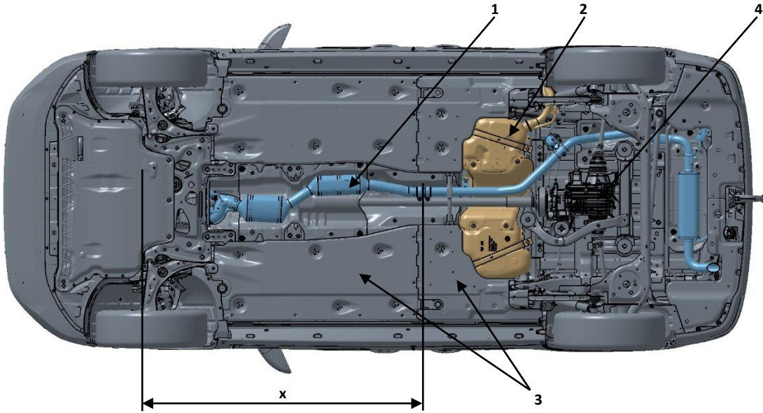
Fig. 1: 4x4 drive exhaust system (all-wheel drive), short wheelbase (illustration: 4x4 drive type, 90KW TDI)
