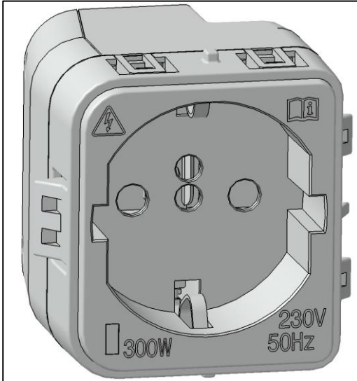
Illustration of the 230-V protective contact socket (PR no. 9Z3)
