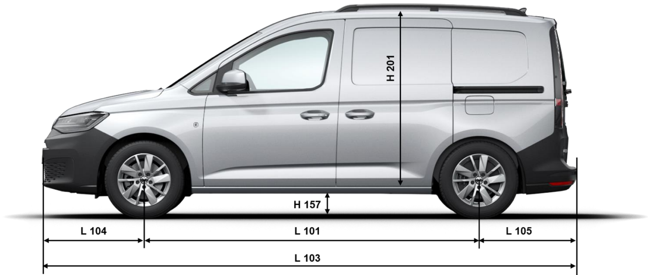
Fig. 1: Vehicle dimensions for Caddy (acc. to DIN 70020, T1)
