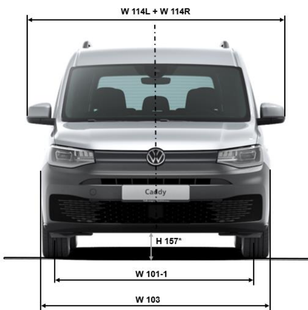
Fig. 3: Vehicle dimensions Caddy/Caddy Maxi, front view (acc. to DIN70020, T1)
