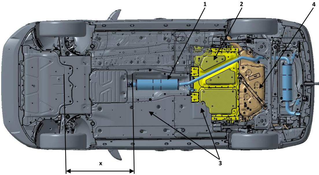
Fig. 1: PHEV exhaust system, short wheelbase (illustration: 4x2 drive type, 85KW TSI)
