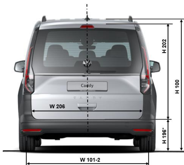
Fig. 4: Vehicle dimensions Caddy/Caddy Maxi, rear view (acc. to DIN70020, T1)
