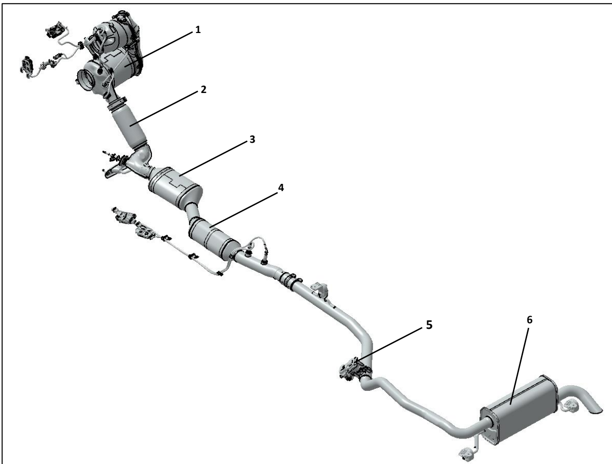
Fig. 3: Emission control with SCR system
