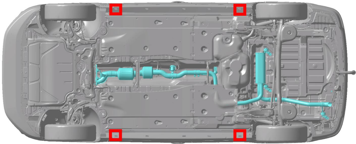
Fig. 1: Positions for jack (schematic diagram)
