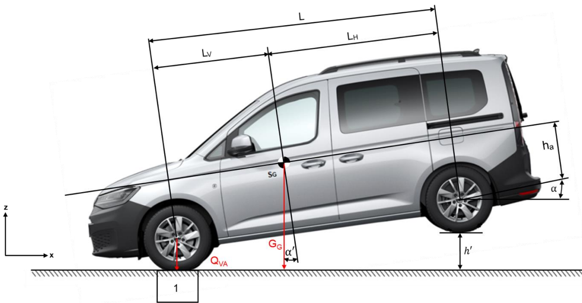
Fig. 2: Determining the location of the vehicle centre of gravity in z-direction
