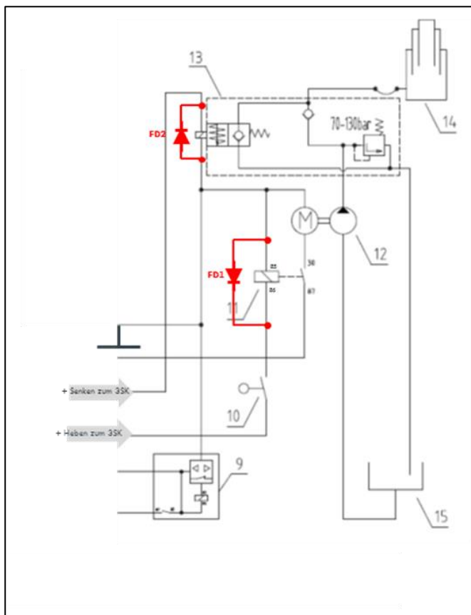
Example of tipper control circuit
